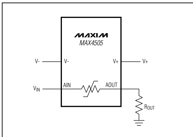
Figure 2. Application Circuit
