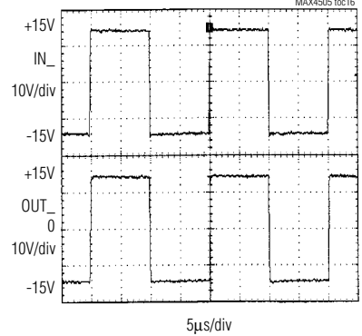
FAULT-FREE RAIL-TO-RAIL SIGNAL HANDLING WITH \pm 15\text{V} SUPPLIES
